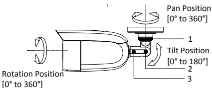
Figure 2-10 3-Axis Adjustment
