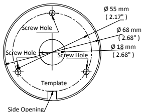
Figure 2-8 Drill Template
