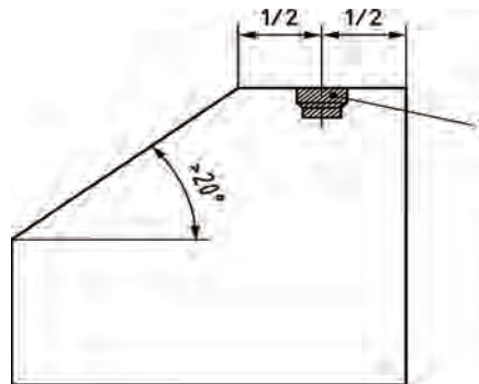
Figure 4 Mounting in rooms with sloping ceiling and horizontal ceiling
